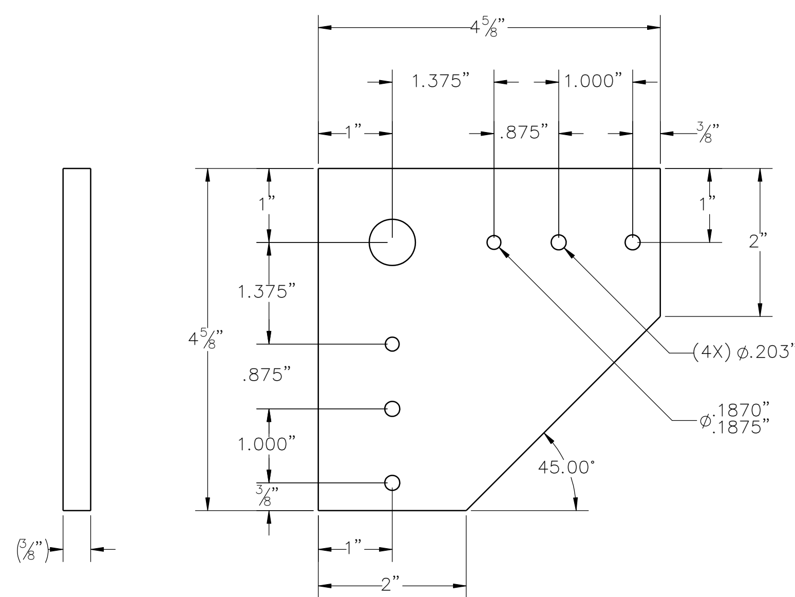
2 CORNER PLATE SCALE: 3/4" = 1"
