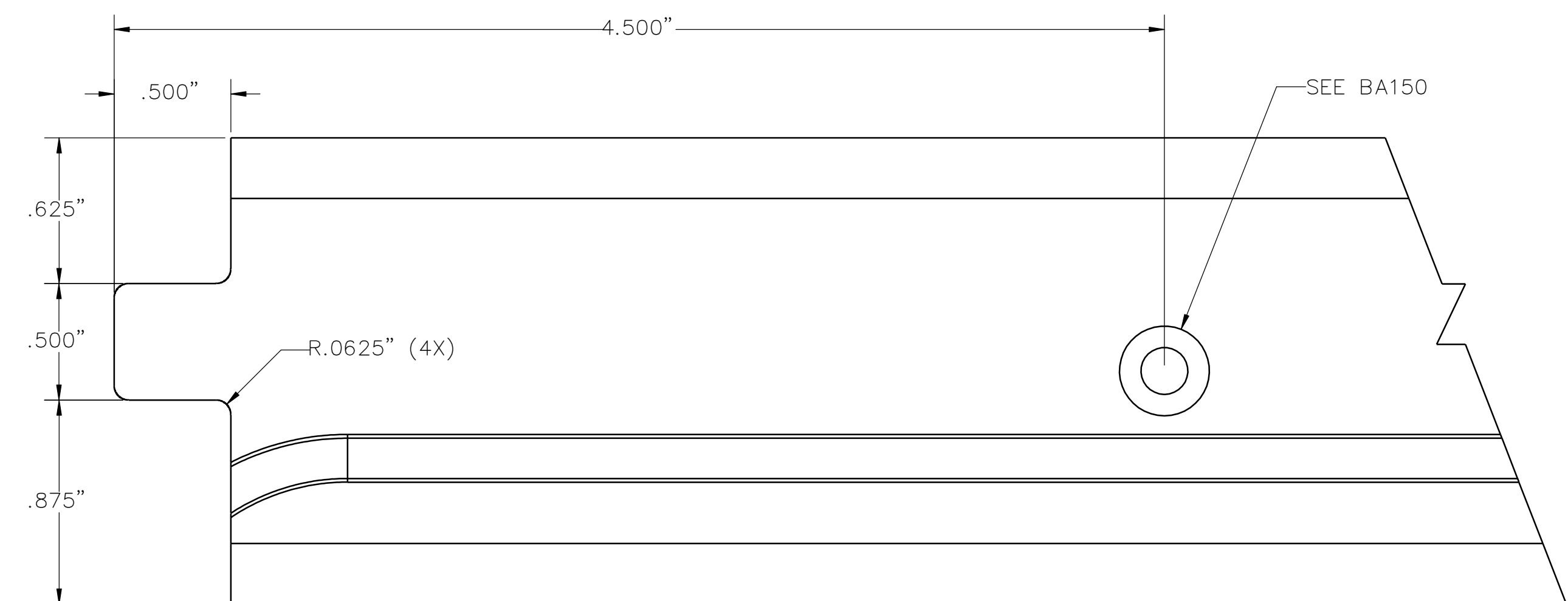
TOP LEFT CONNECTION SCALE: 2:1
