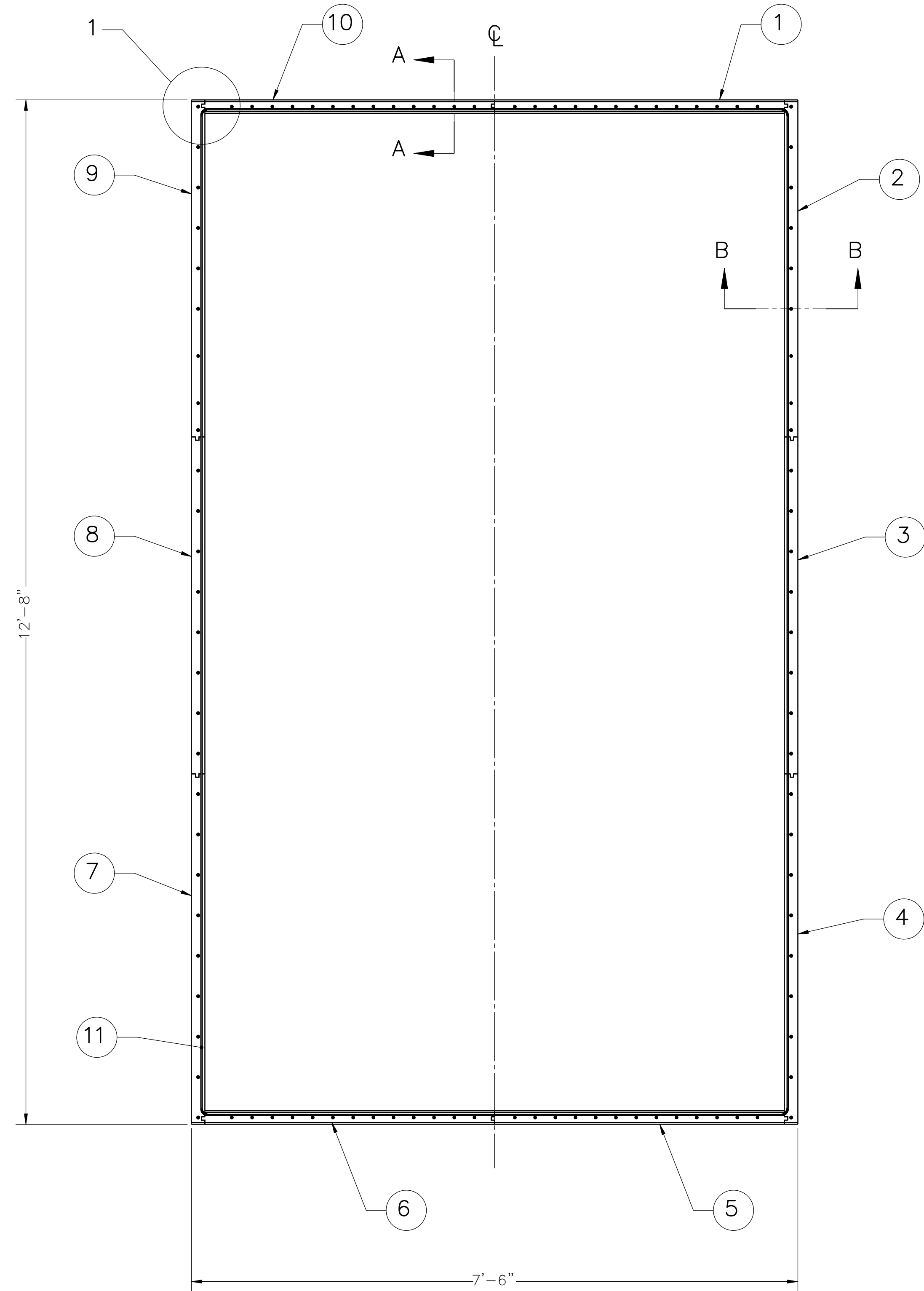
HEADGATE SEAL ASSEMBLY SCALE: 1" = 1'-0"
