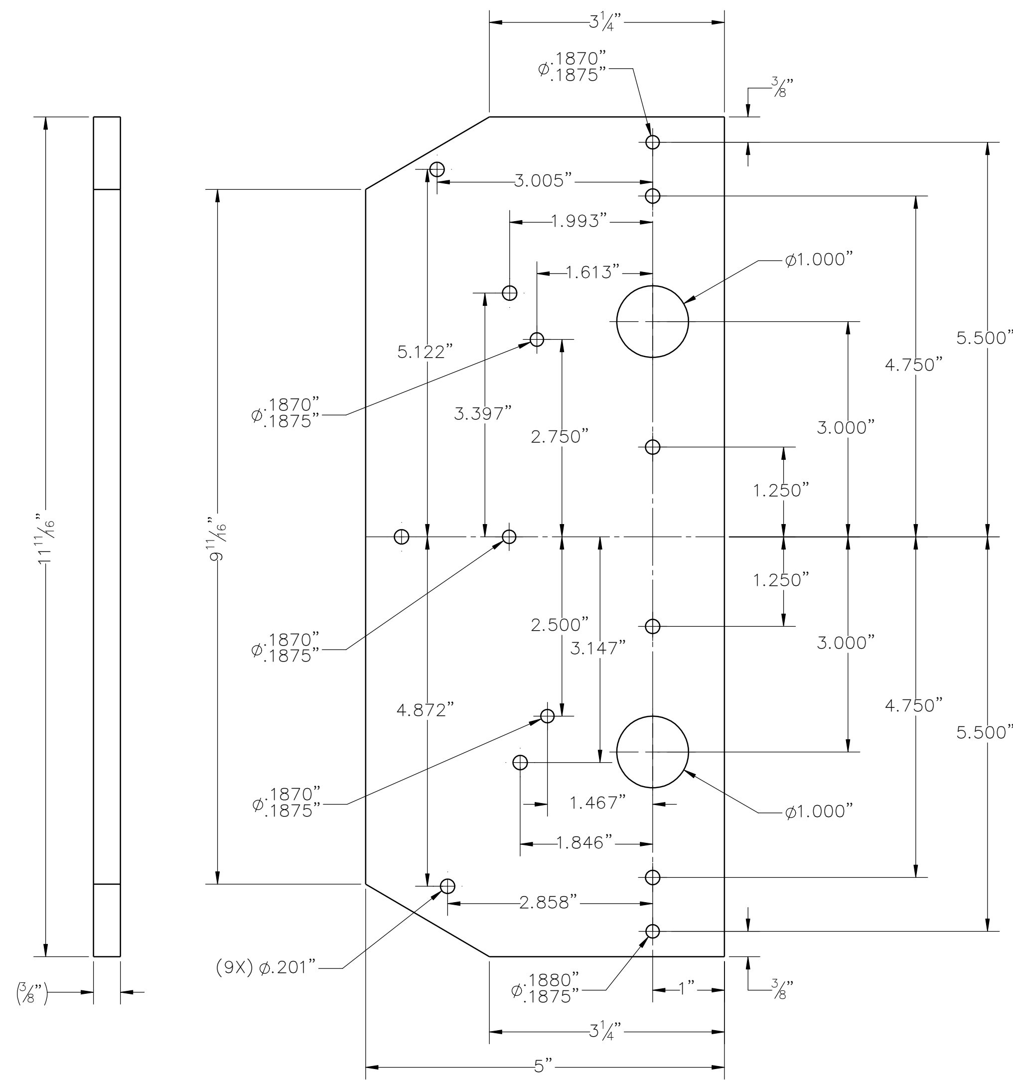
5 SIDE PLATE SCALE: 3/4" = 1"
