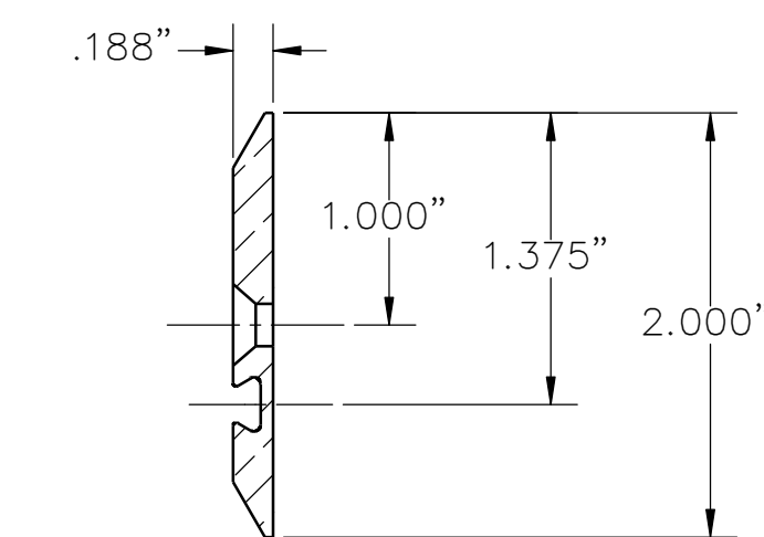
SECTION C-C
